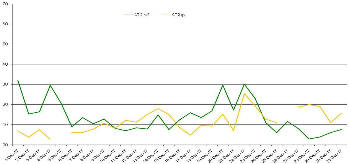
PM2.5 nef si PM2.5 gv (ug/m3), perioada: 01 Decemb 2017-31 Decemb 2017 - Date validate
